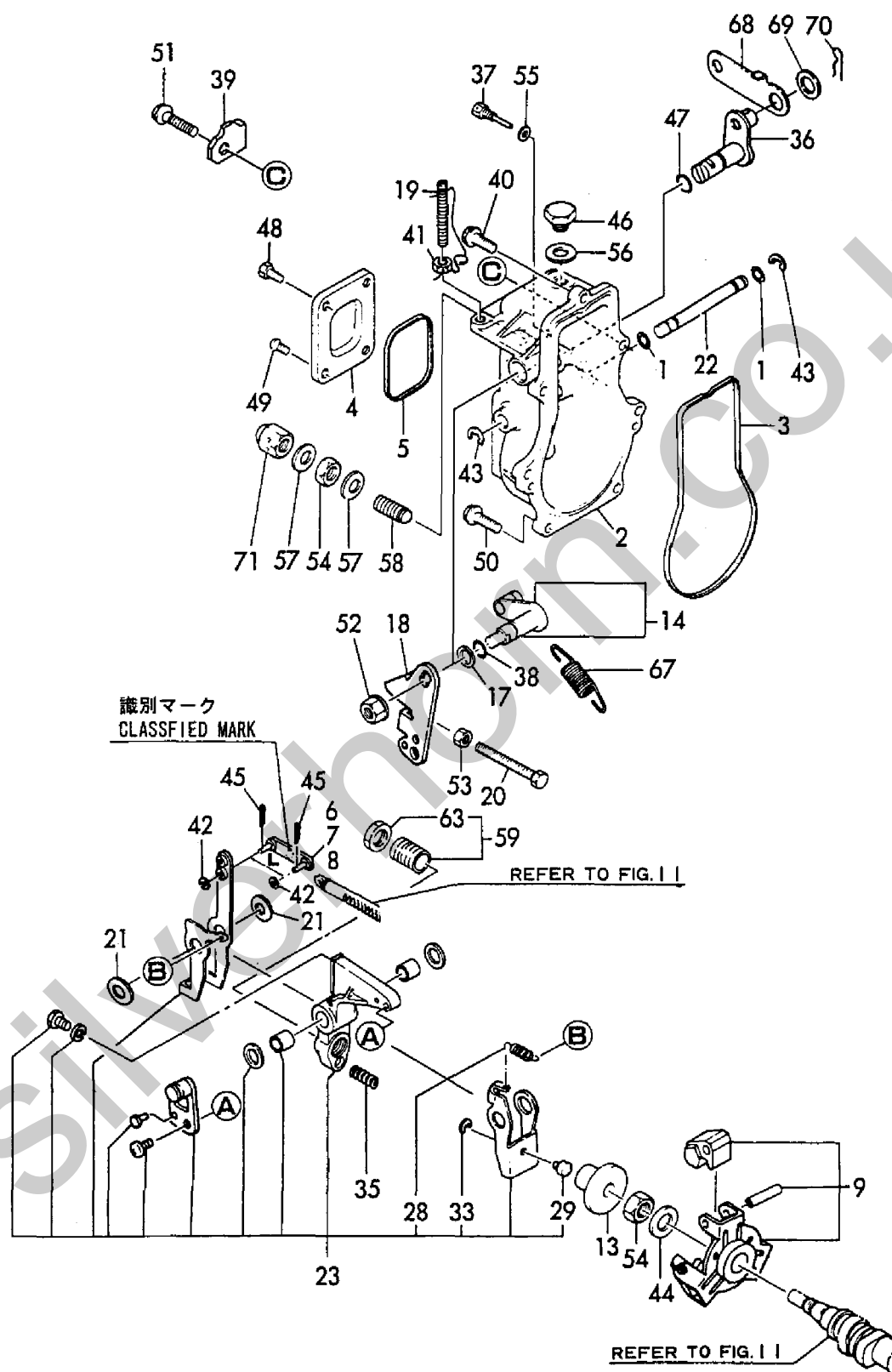
Fig. 12 ガバナ GOVERNOR
