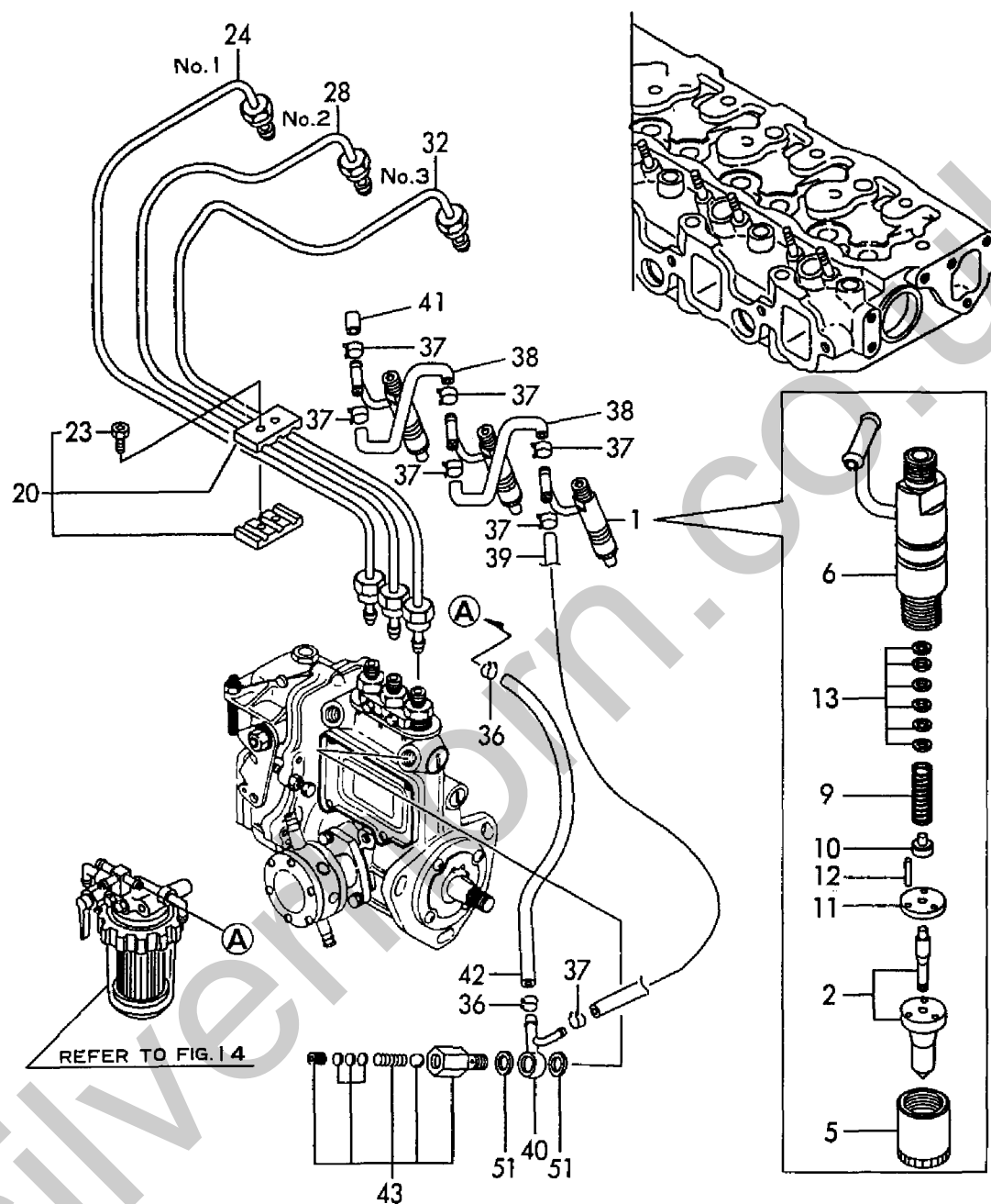
Fig. 13 燃料噴射弁 FUEL INJECTION VALVE
